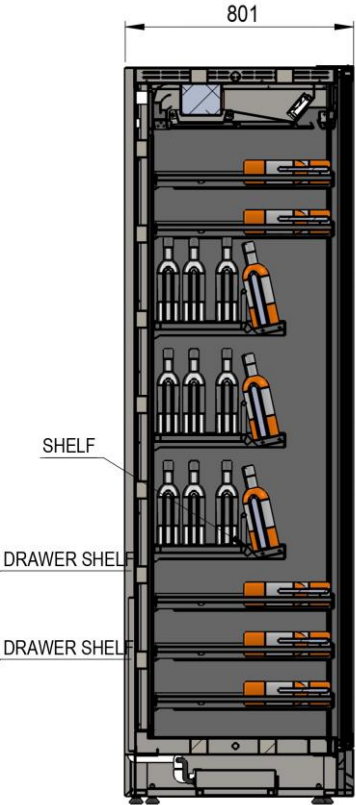
SECTION G-G
