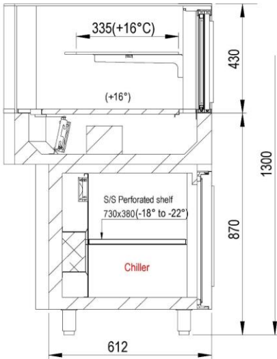
SECTION C-C SCALE 1 : 15
