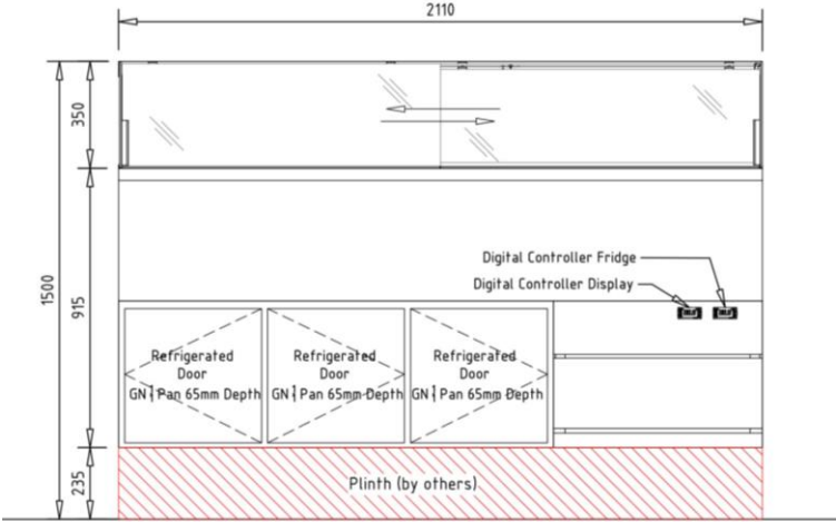
ELEVATION A (Operator side)
