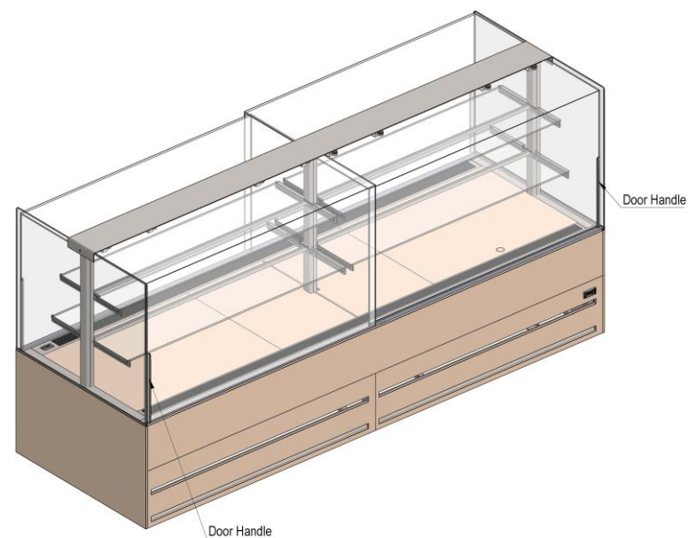
Operator Side View
